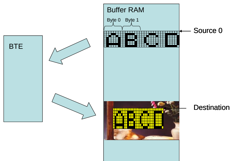
Figure 13-33 : Hardware Data Flow
