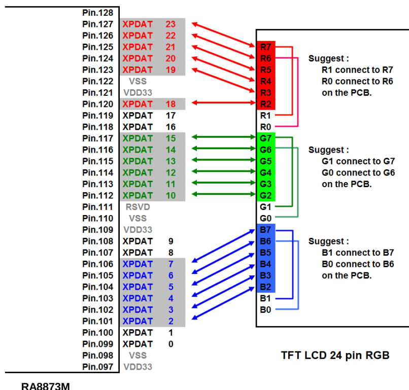
Figure 10-2 : RA8873M color depth 18bit with LCD panel pin connect
