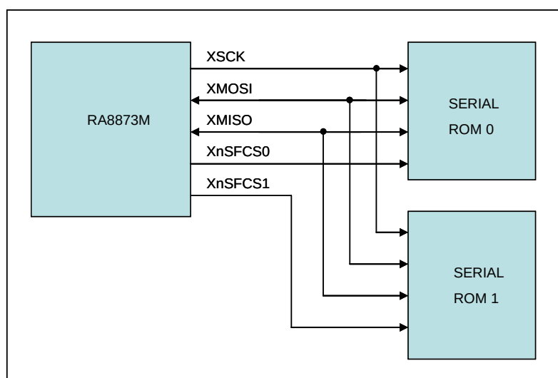
Figure 16-3 : RA8873M Serial Flash/ROM System
