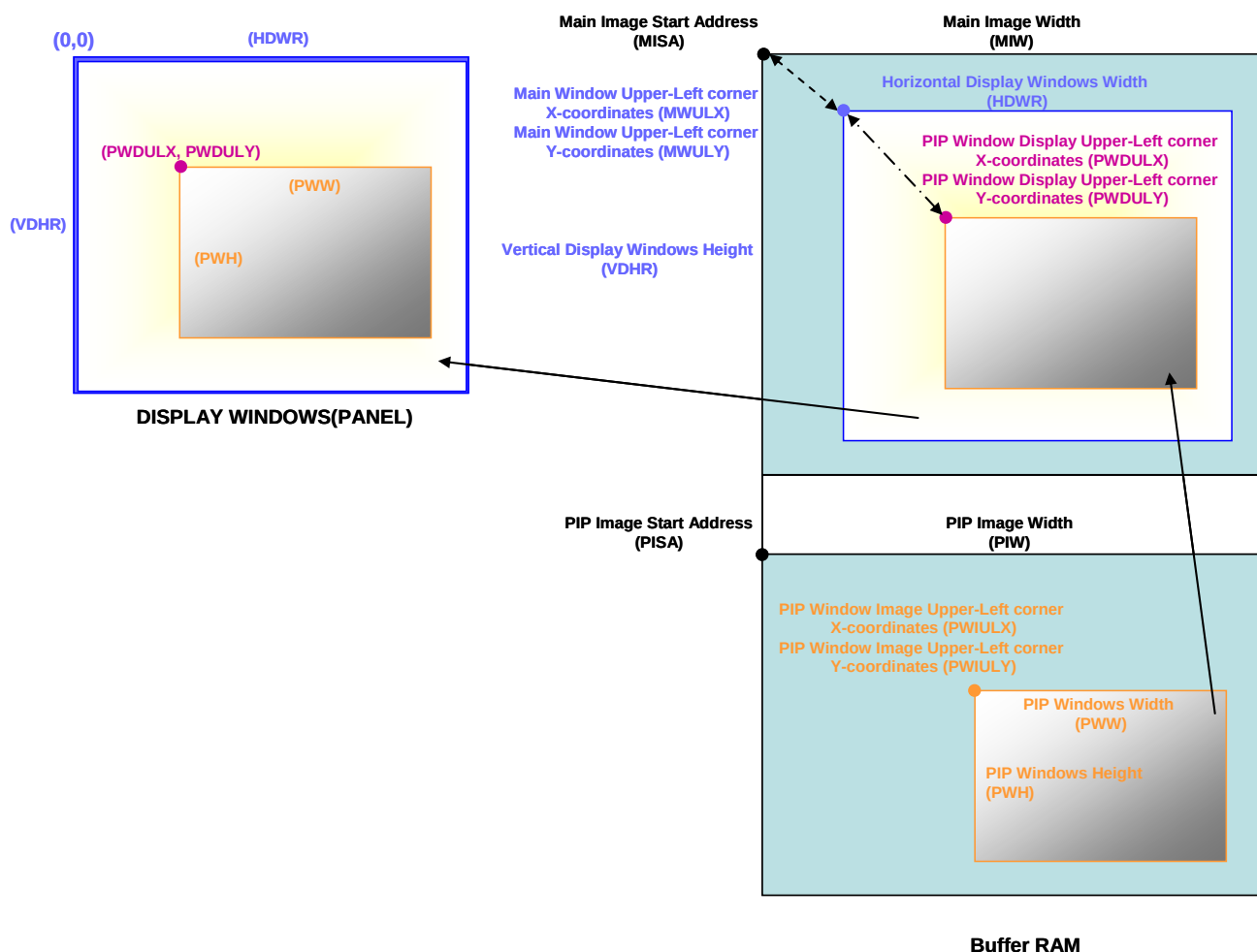
Figure 19-2 : LCD Display
