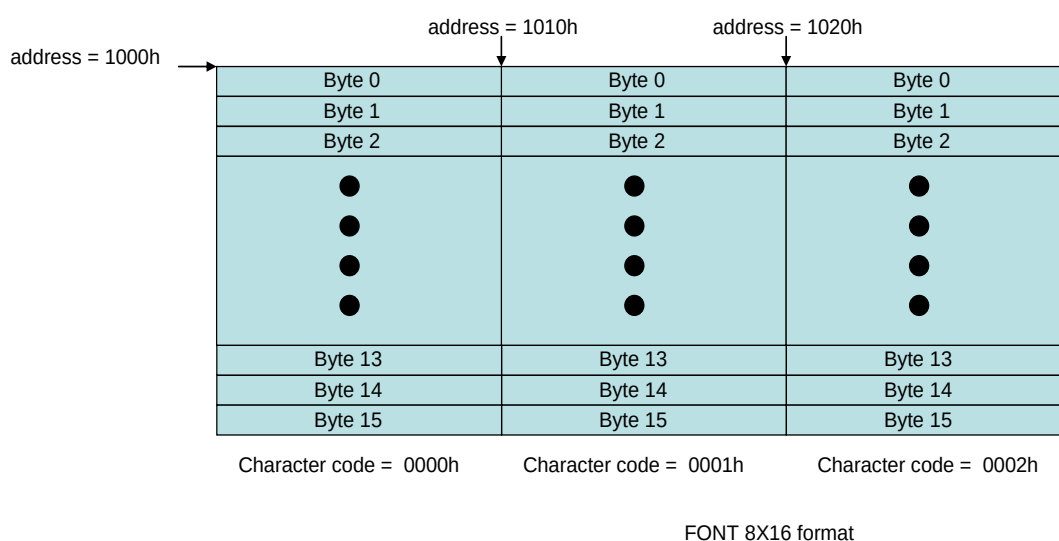
Figure 14-4 : Font 8X16 Array in Buffer RAM
