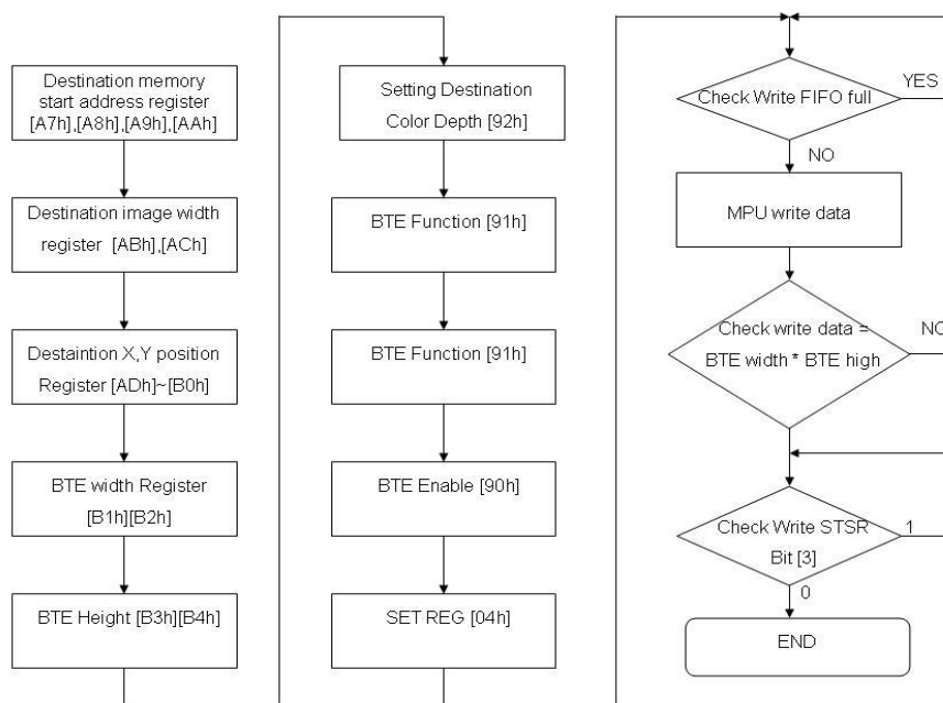
Figure 13-20 : Flow Chart
