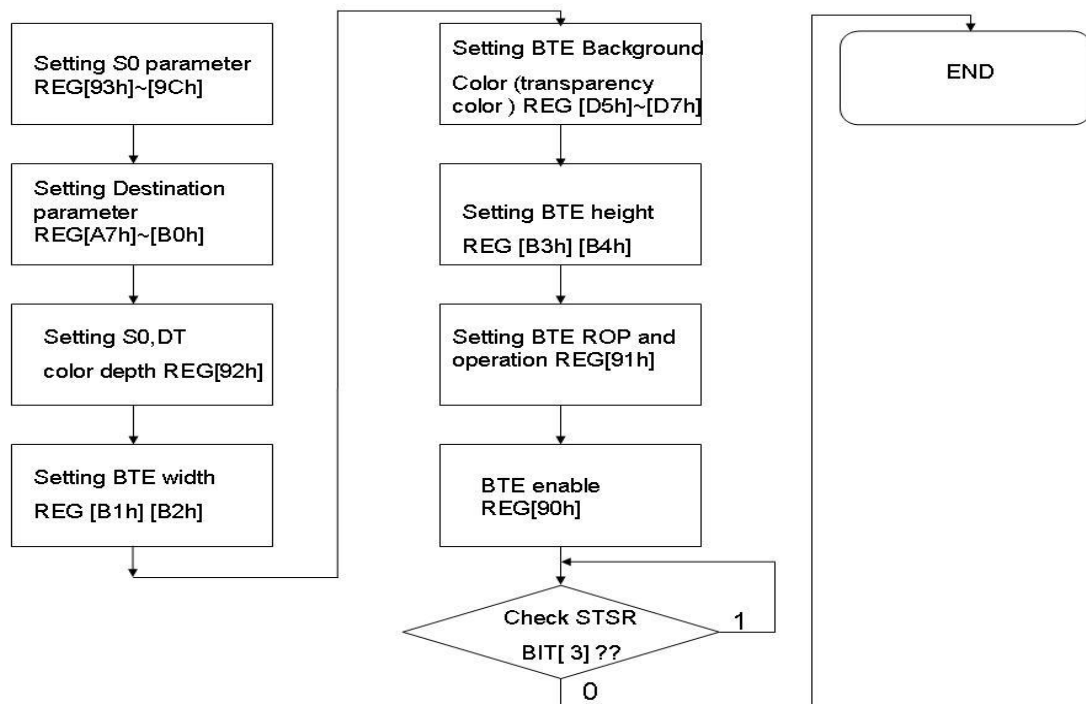
Figure 13-12 : Flow Chart
