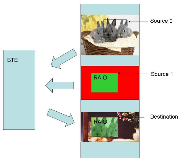
Figure 13-27 : 16bpp Pixel Mode Hardware Data Flow
