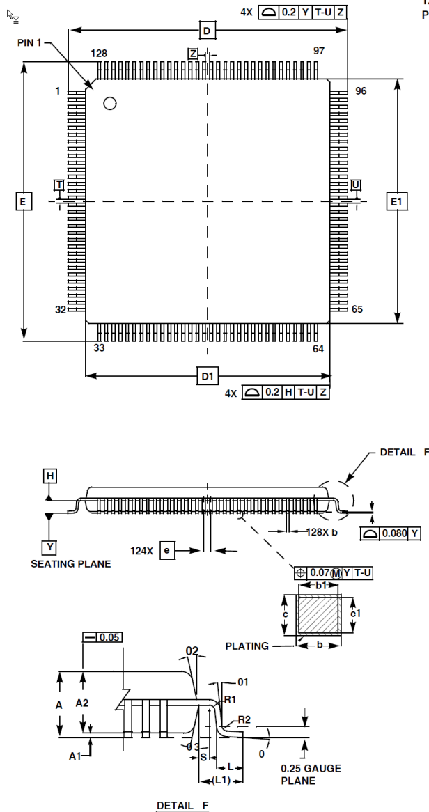
Figure 3-2 : RA8873M Package Outline Dimensions
