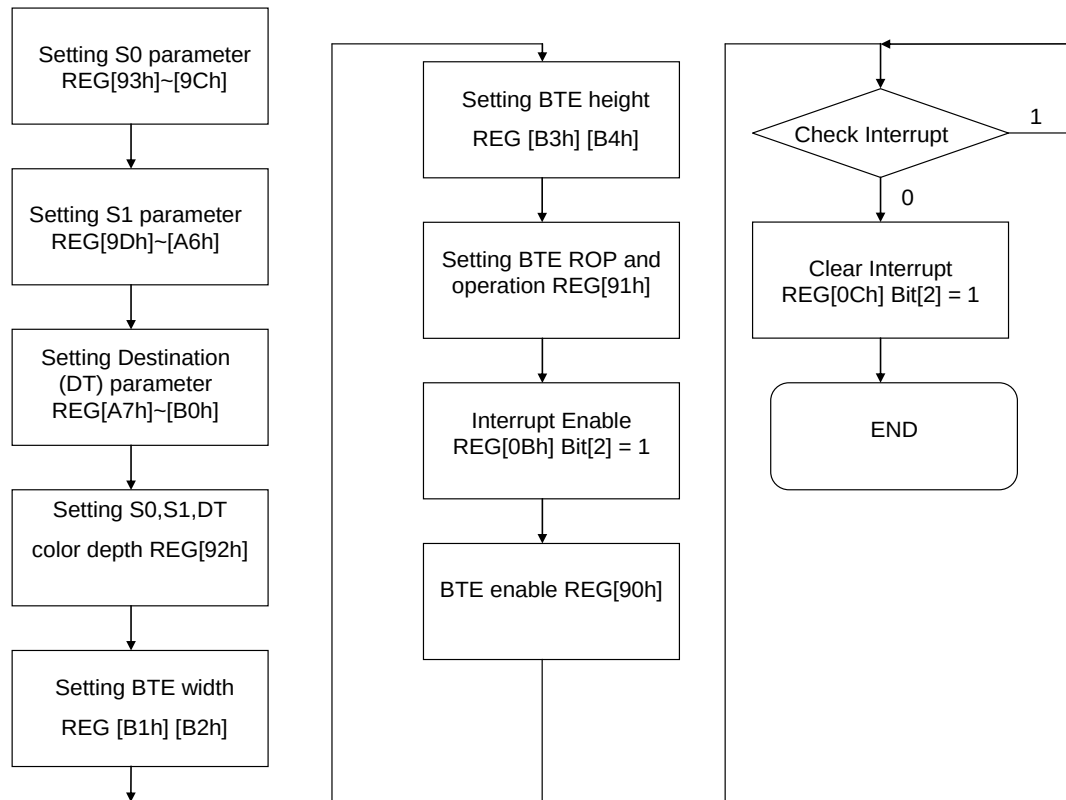
Figure 13-9 : Flow Chart – Check Int
