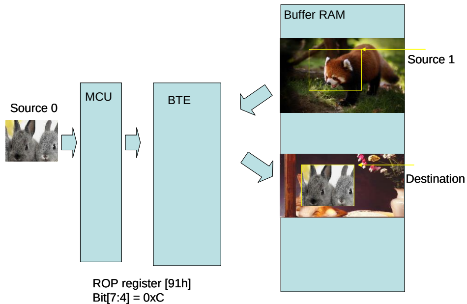
Figure 13-5 : Hardware Data Flow
