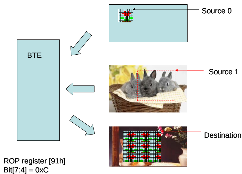
Figure 13-16 : Hardware Data Flow
