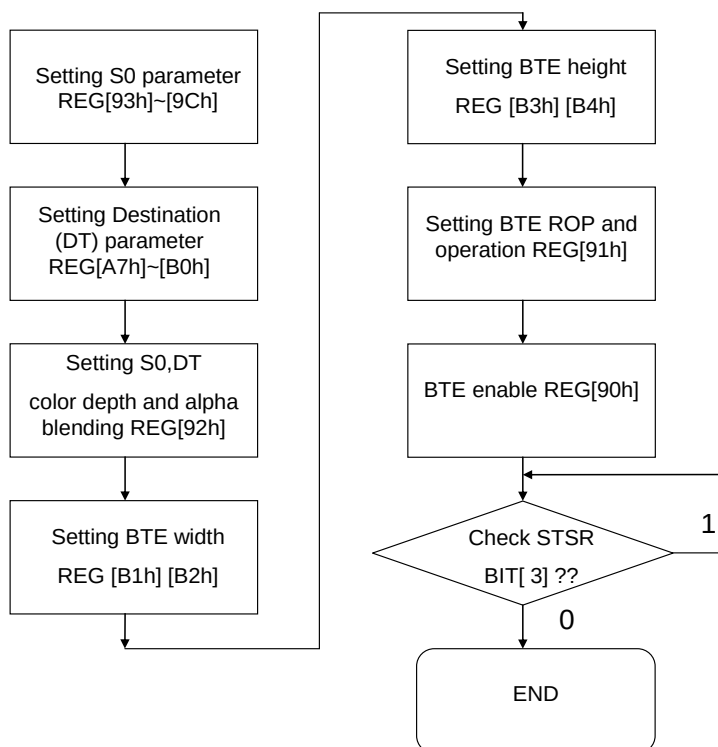
Figure 13-36 : Flow Chart
