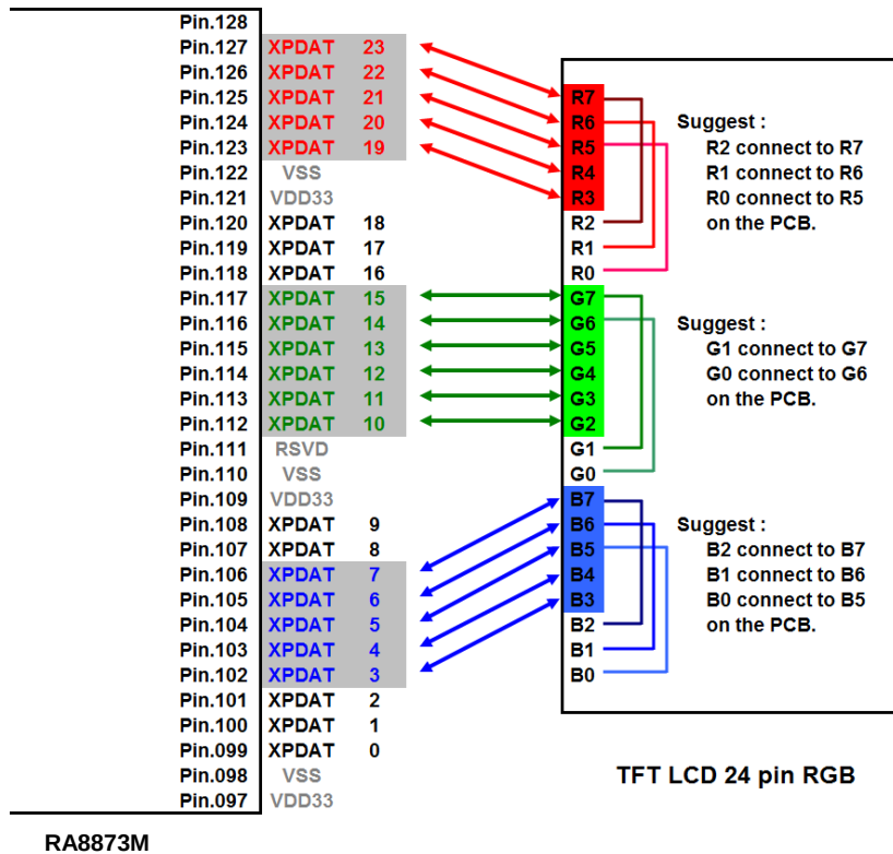
Figure 10-3 : RA8873M color depth 16bit with LCD panel pin connect
