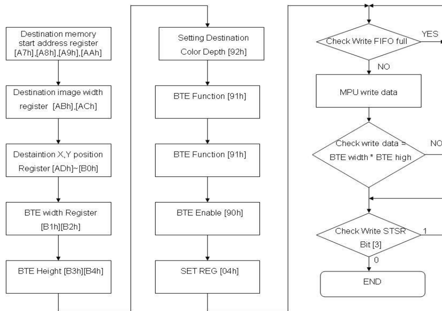
Figure 13-25 : Flow Chart
