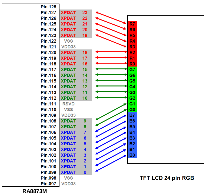
Figure 10-1 : RA8873M color depth 24bit with LCD panel pin connect
