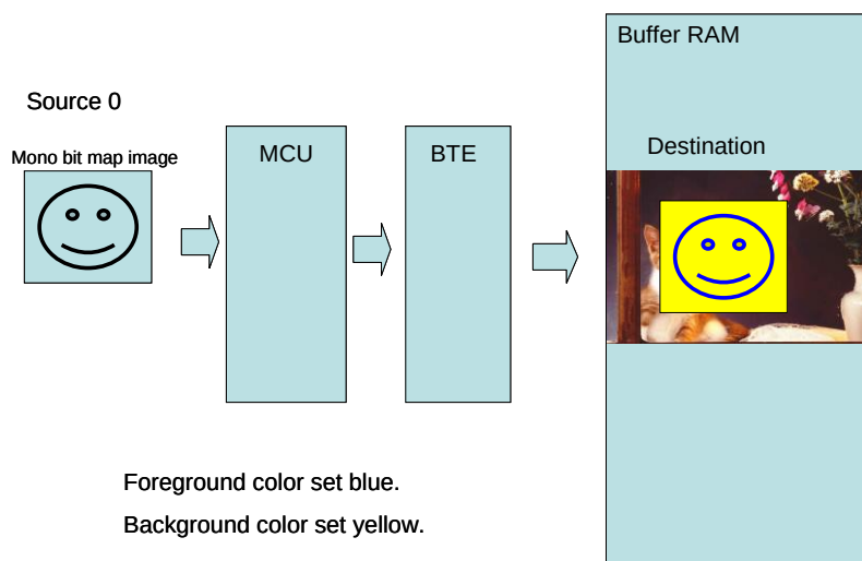
Figure 13-19 : Hardware Data Flow
